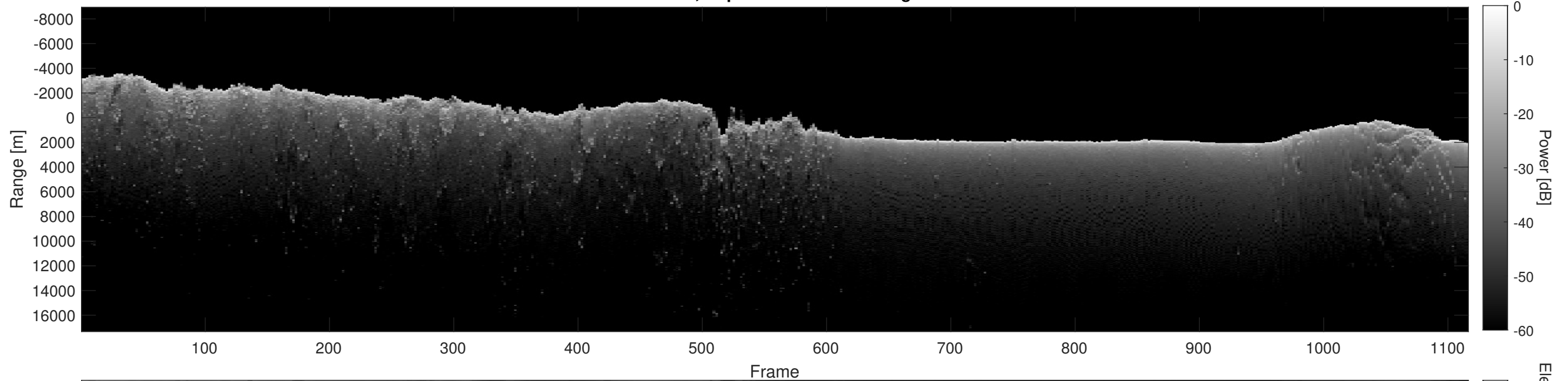
Orbit 12137, Depth-Corrected Cluttergram
