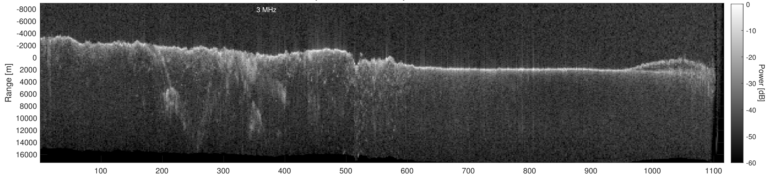
Orbit 12137, Depth-Corrected Cluttergram
