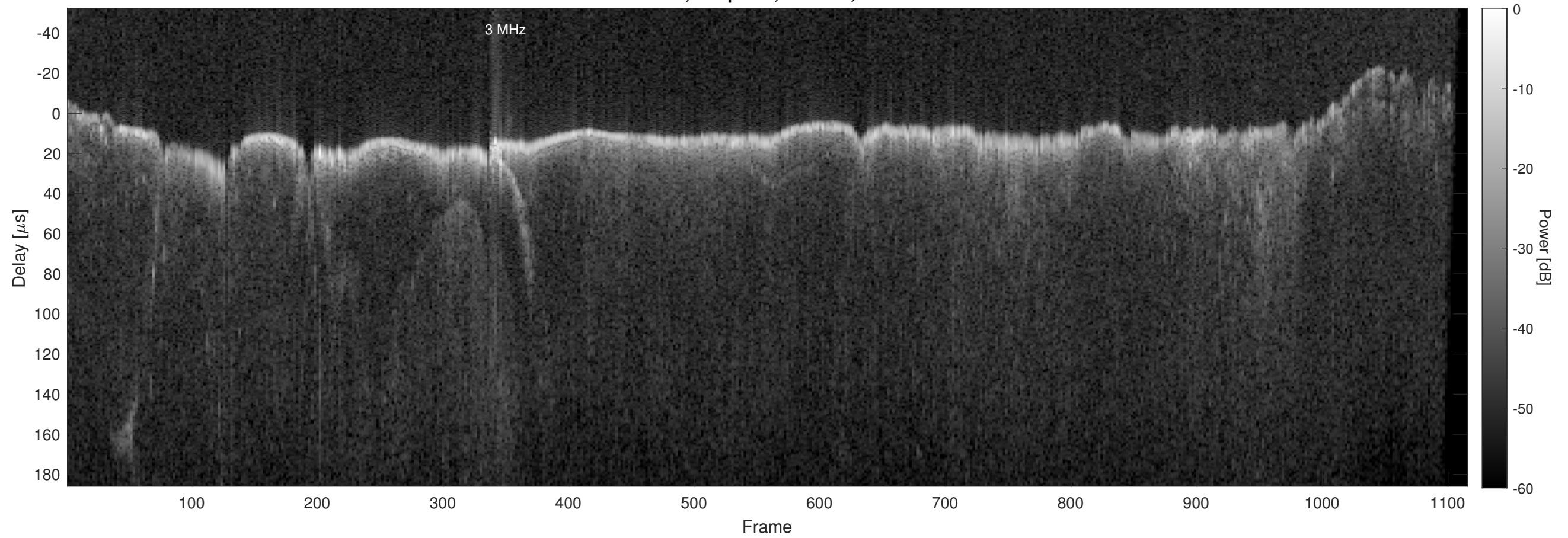
Orbit 12139, Chapman, Window, Channel 2
