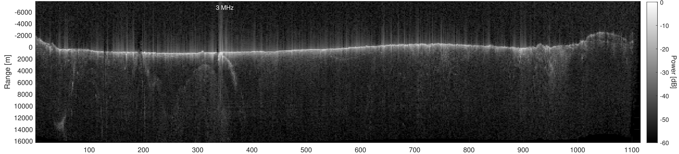
Orbit 12139, Depth-Corrected Cluttergram
