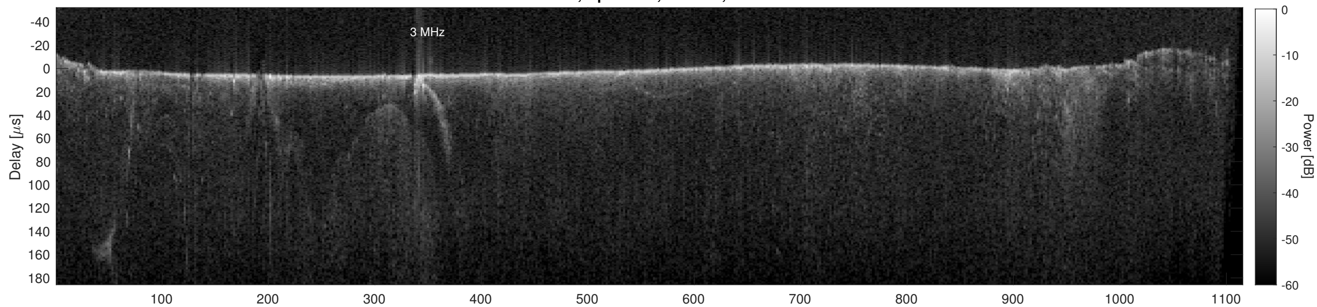
Orbit 12139, Cluttergram
