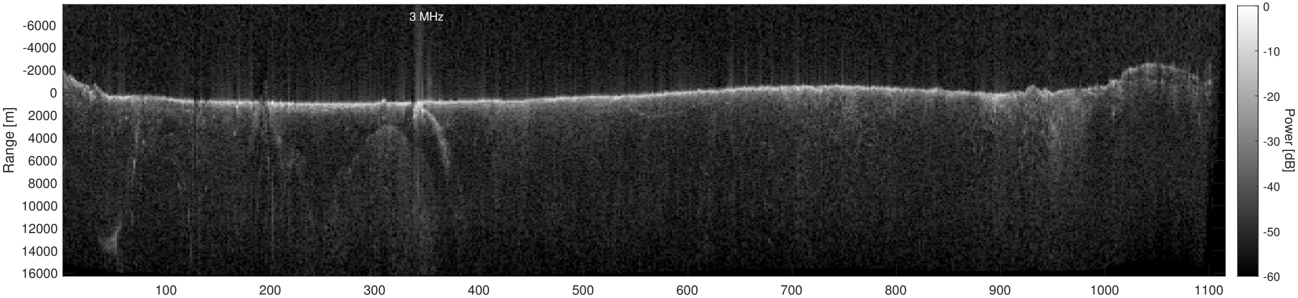
Orbit 12139, Depth-Corrected Cluttergram
