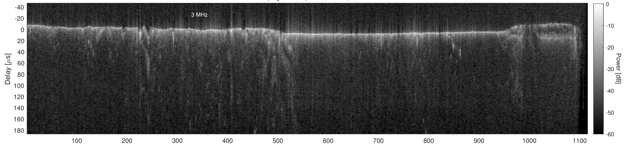
Orbit 12141, Cluttergram
