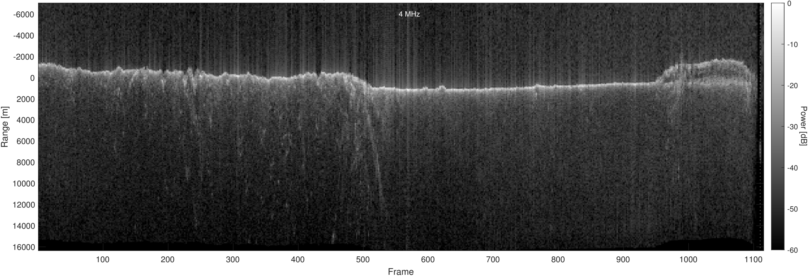
Orbit 12141, Optimized, No Window, Depth-Corrected, Channel 2
