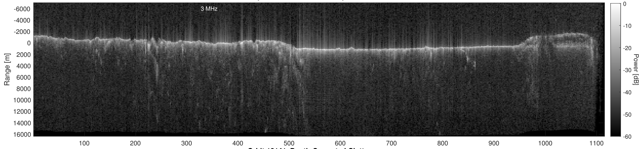
Orbit 12141, Depth-Corrected Cluttergram
