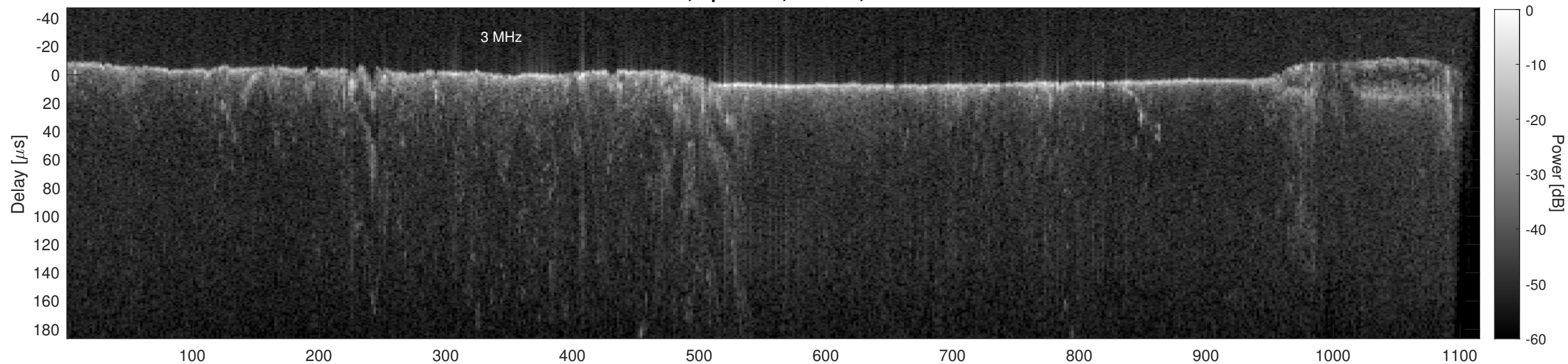
Orbit 12141, Cluttergram
