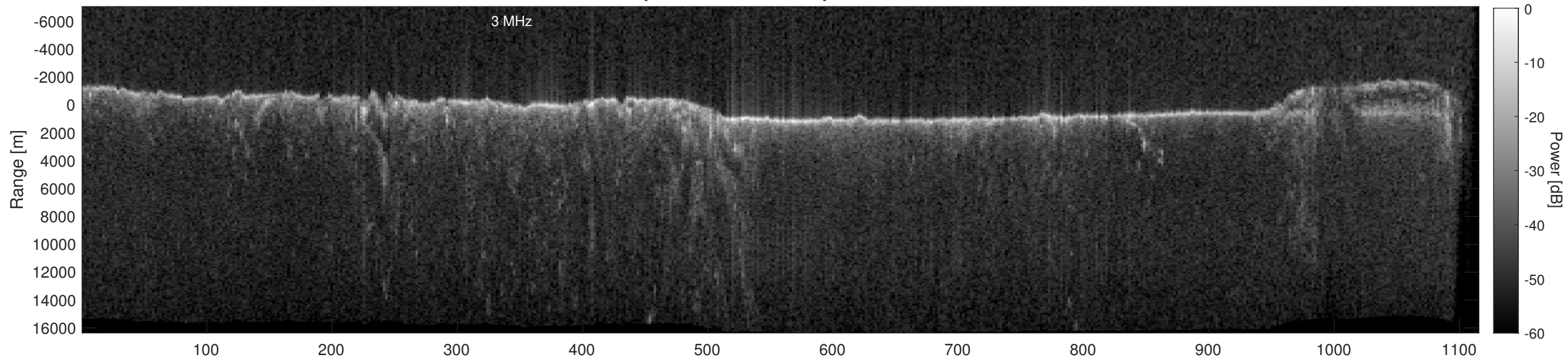
Orbit 12141, Depth-Corrected Cluttergram
