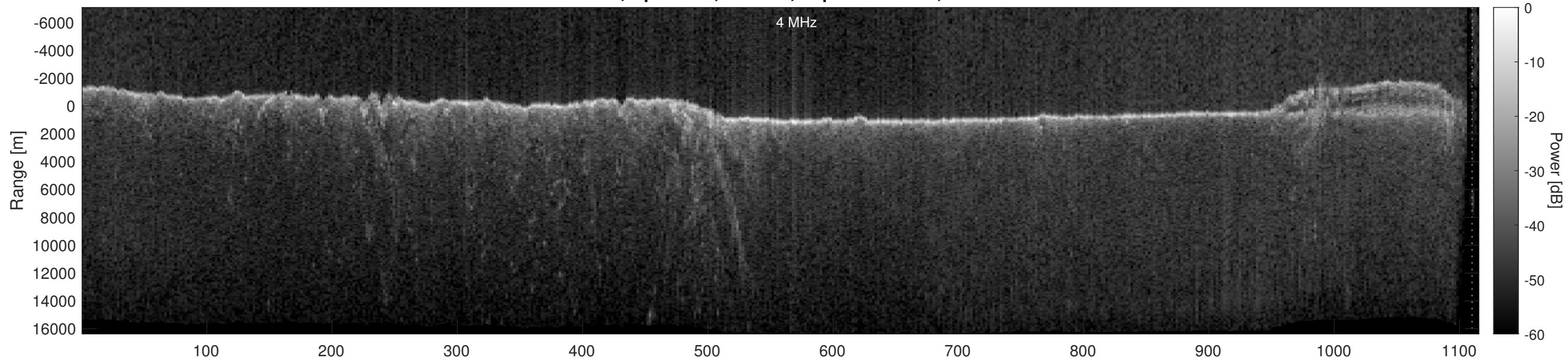
Orbit 12141, Optimized, Window, Depth-Corrected, Channel 2
