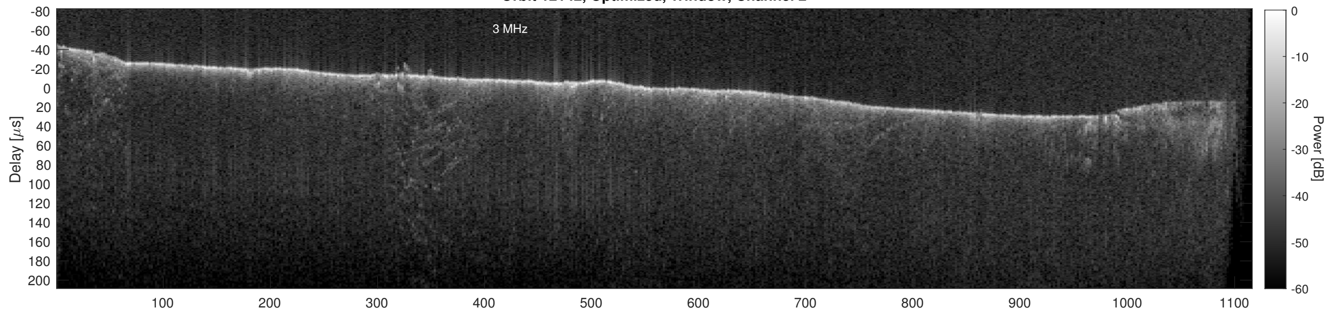
Orbit 12142, Cluttergram
