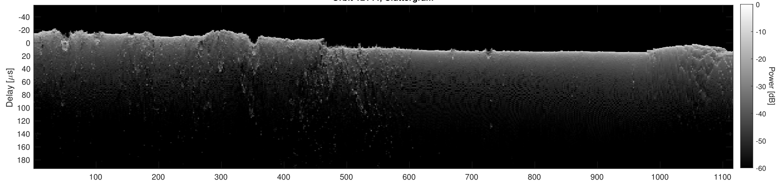
Orbit 12144, Cluttergram
