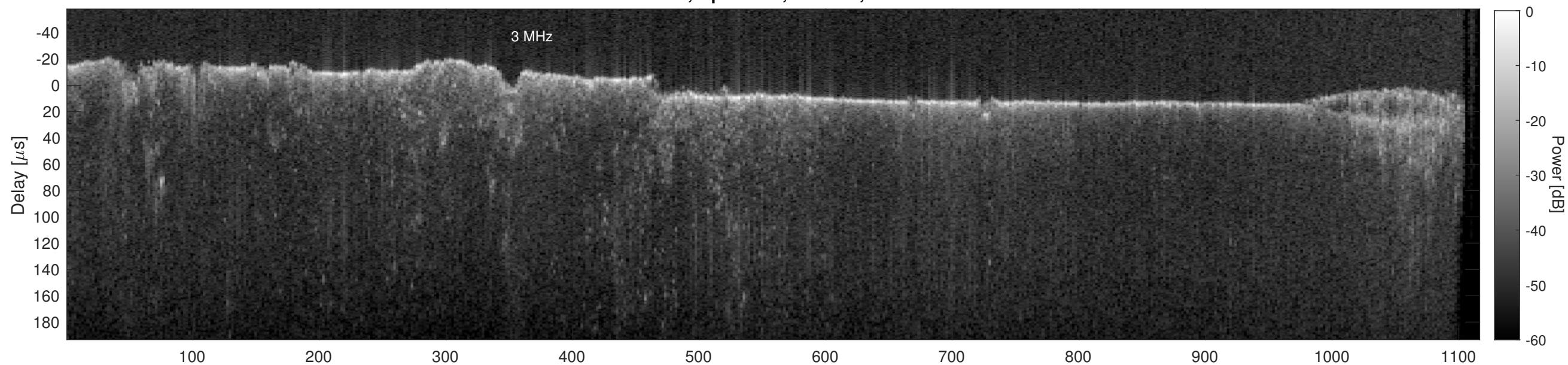
Orbit 12144, Cluttergram
