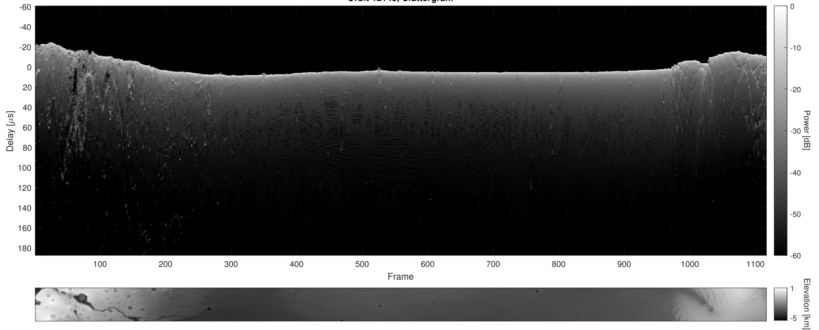
Orbit 12145, Cluttergram
