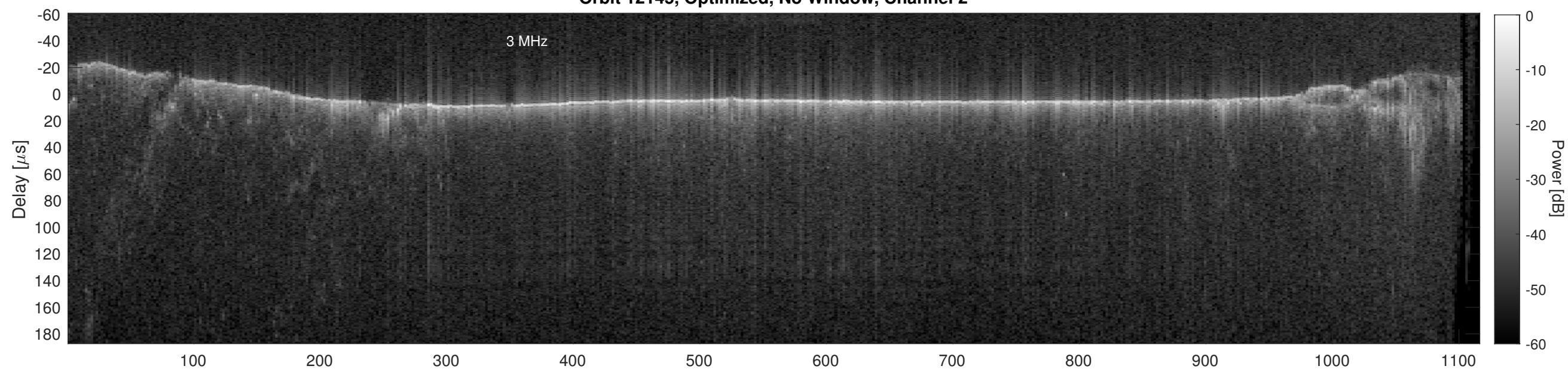
Orbit 12145, Cluttergram
