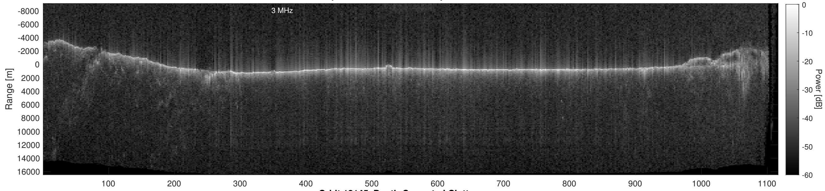
Orbit 12145, Depth-Corrected Cluttergram
