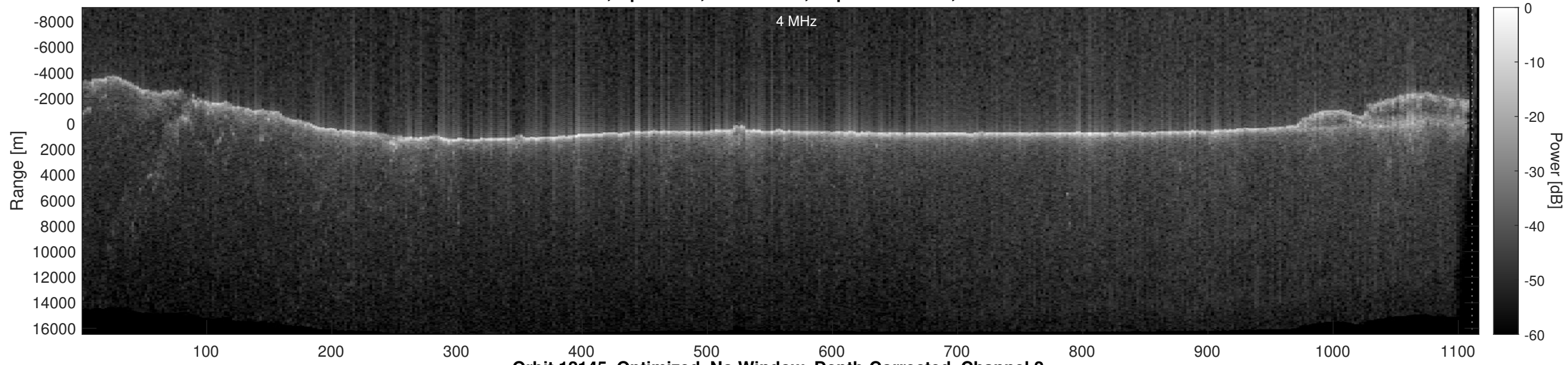
Orbit 12145, Optimized, No Window, Depth-Corrected, Channel 2
