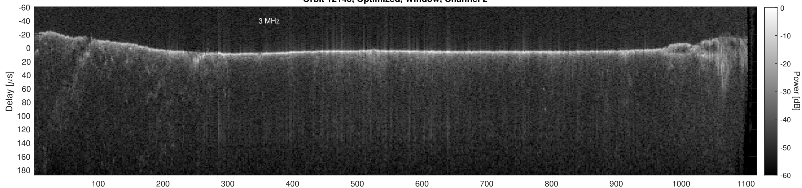
Orbit 12145, Cluttergram
