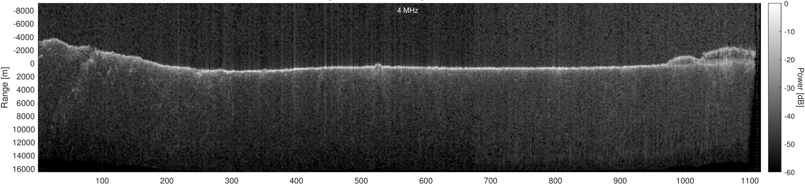
Orbit 12145, Optimized, Window, Depth-Corrected, Channel 2
