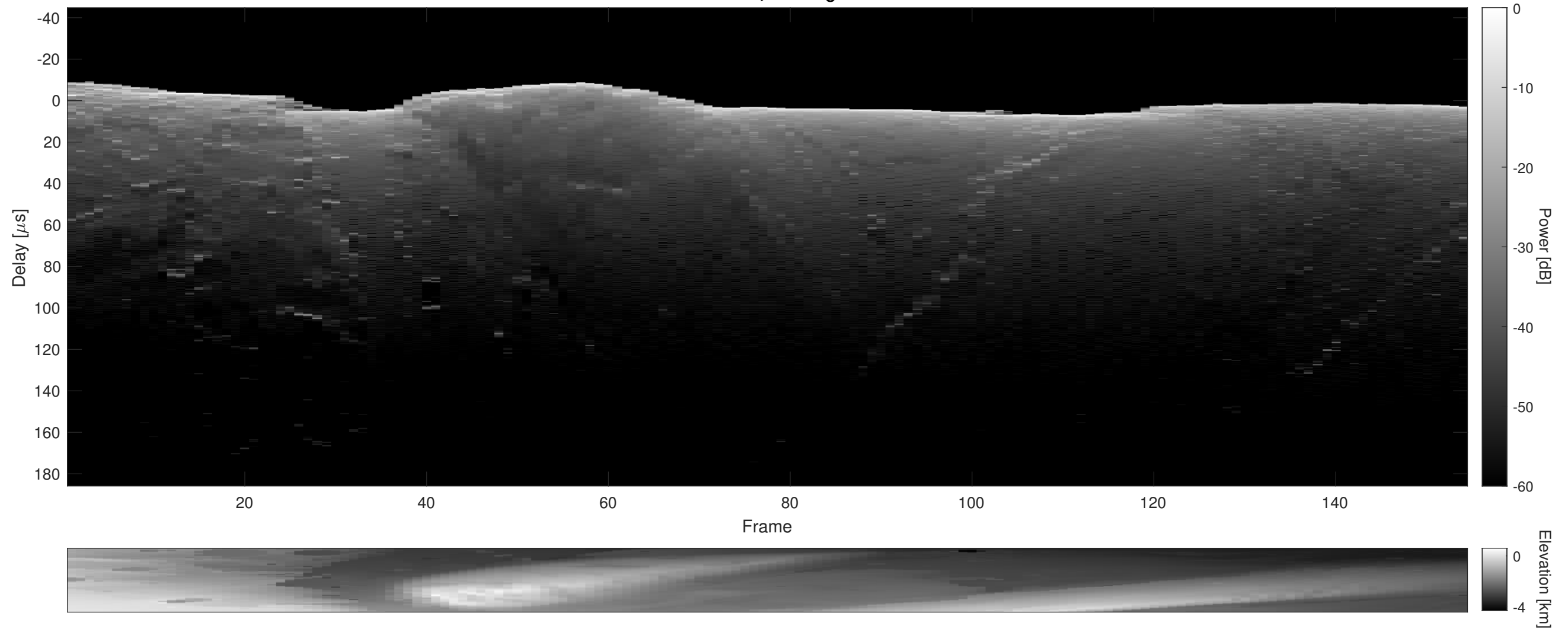
Orbit 12146, Cluttergram
