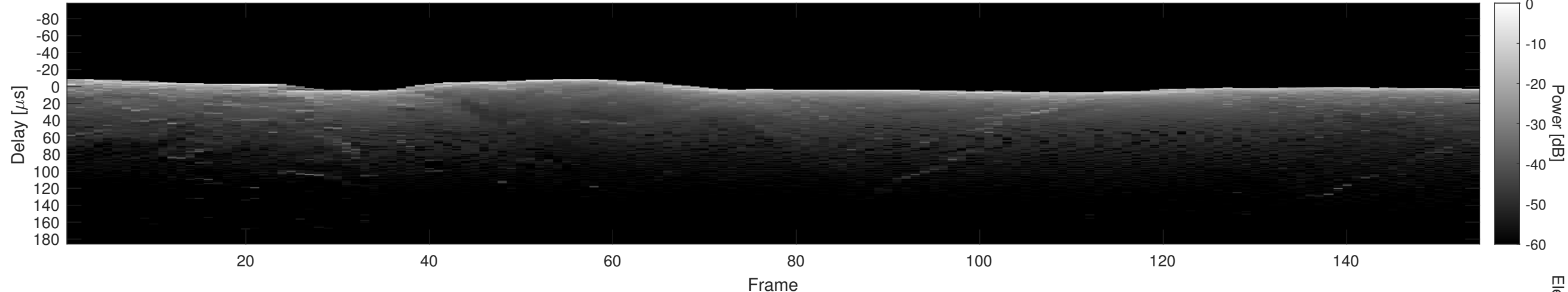
Orbit 12146, Cluttergram
