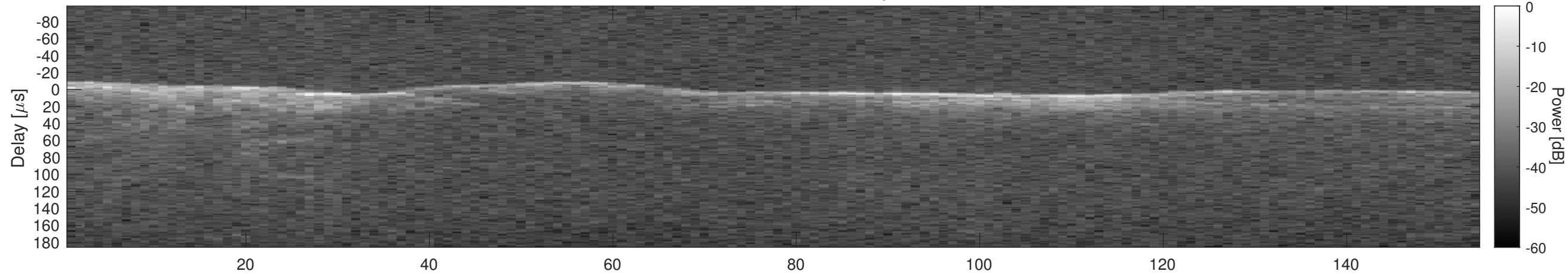
Orbit 12146, Cluttergram
