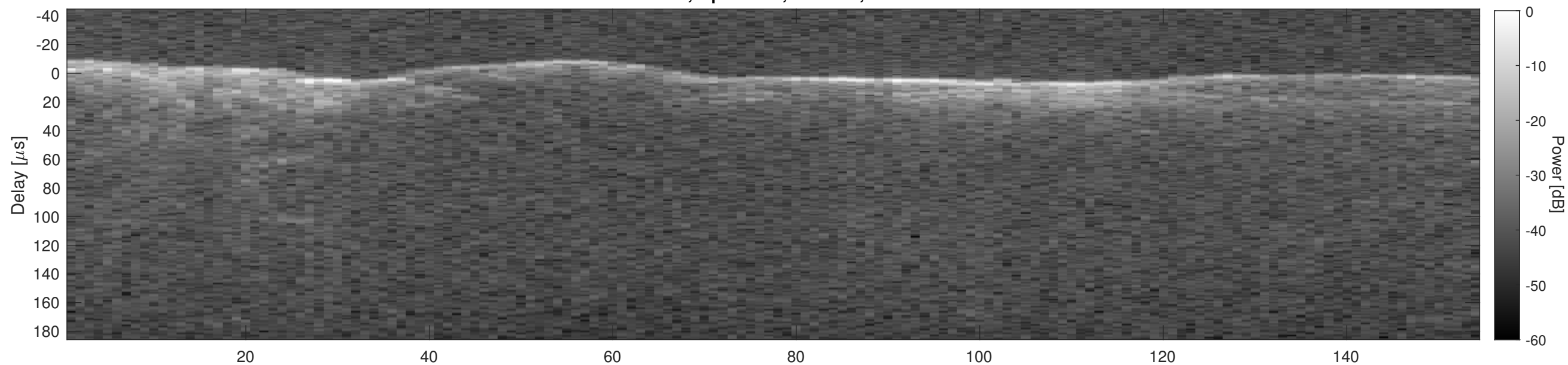
Orbit 12146, Cluttergram
