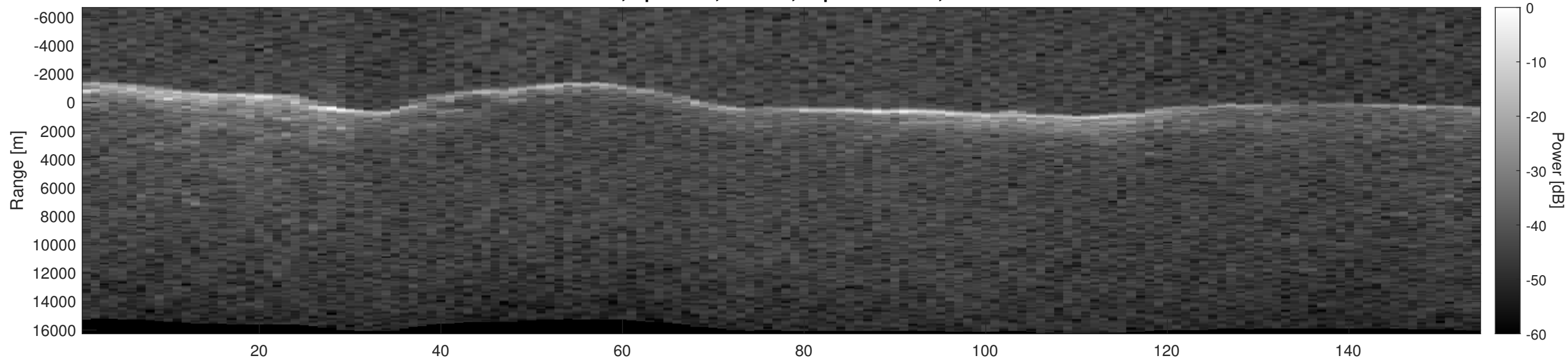
Orbit 12146, Optimized, Window, Depth-Corrected, Channel 2
