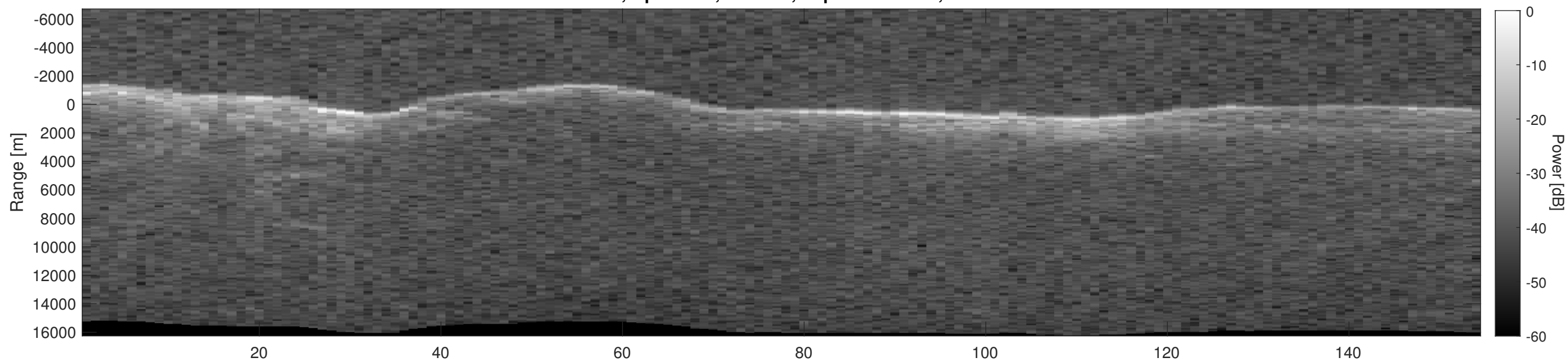
Orbit 12146, Depth-Corrected Cluttergram
