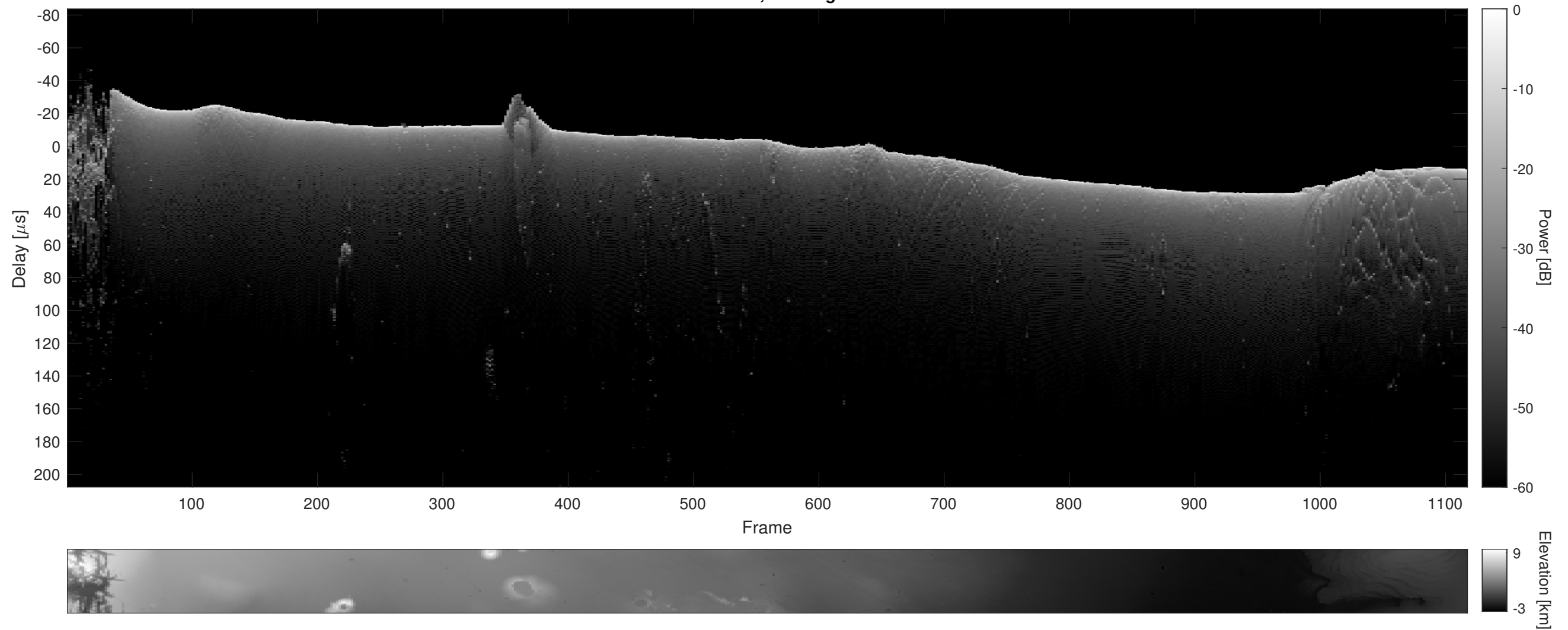
Orbit 12149, Cluttergram
