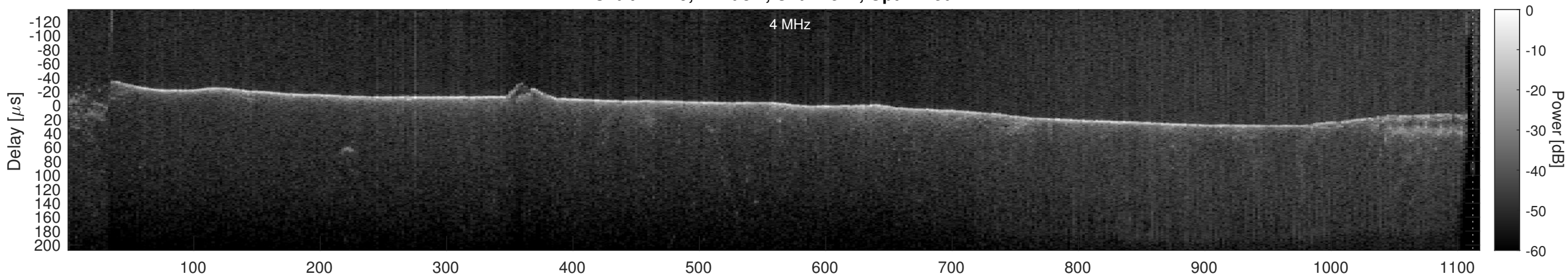
Orbit 12149, Cluttergram
