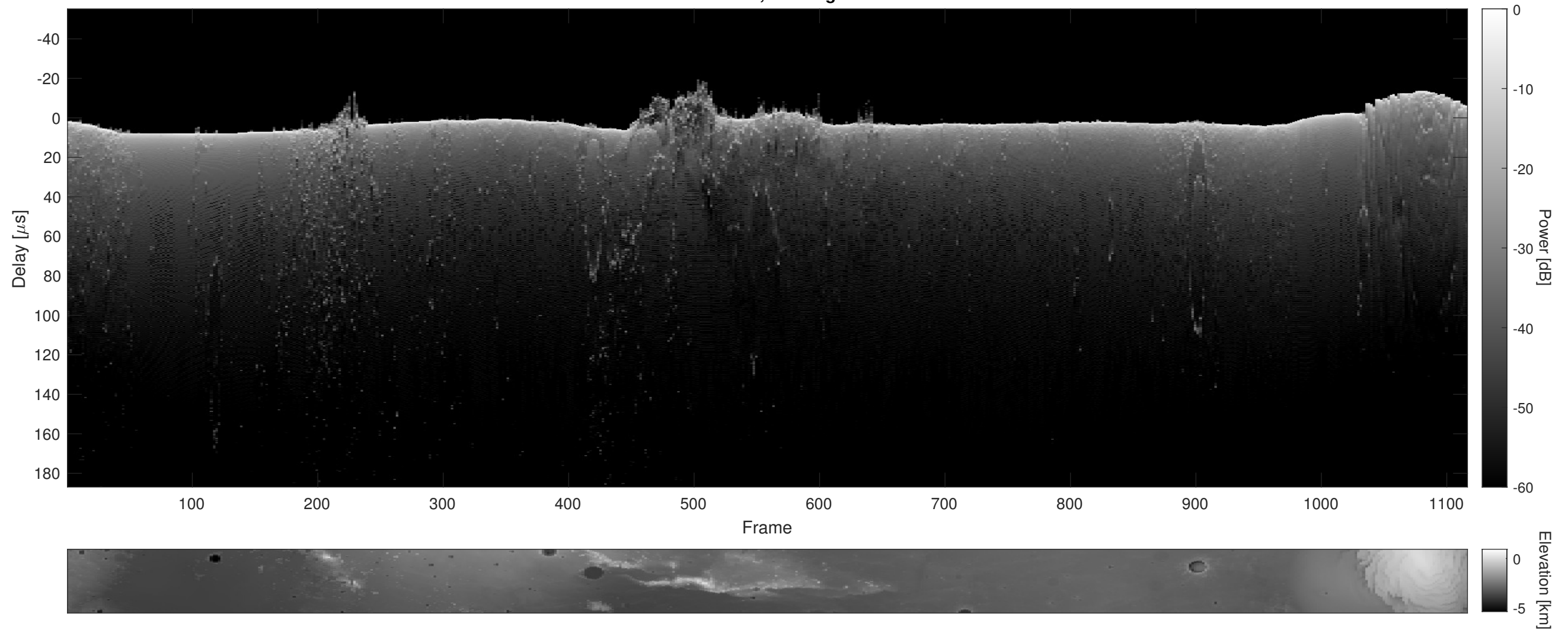
Orbit 12150, Cluttergram
