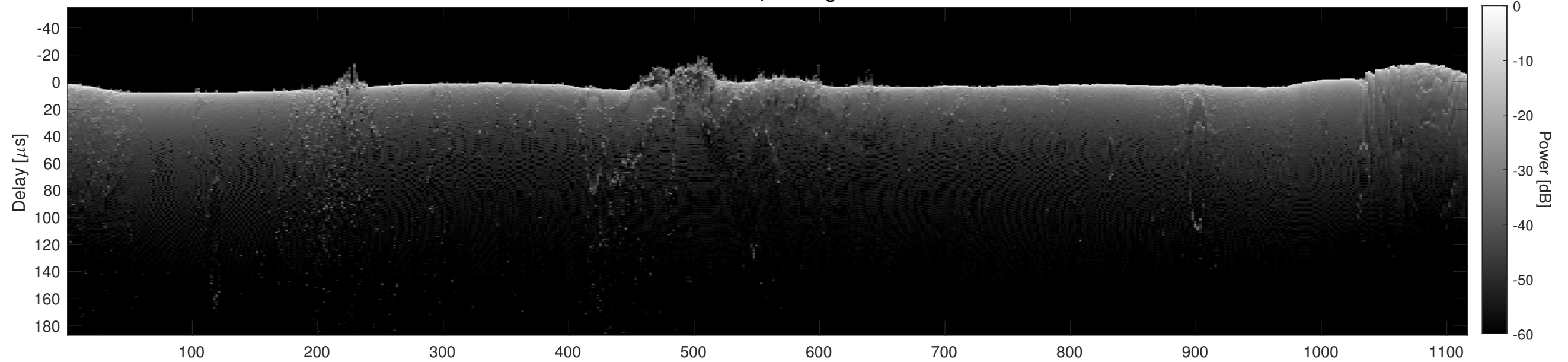
Orbit 12150, Cluttergram
