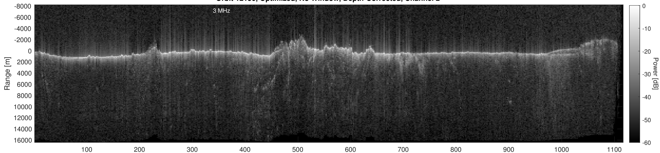
Orbit 12150, Depth-Corrected Cluttergram
