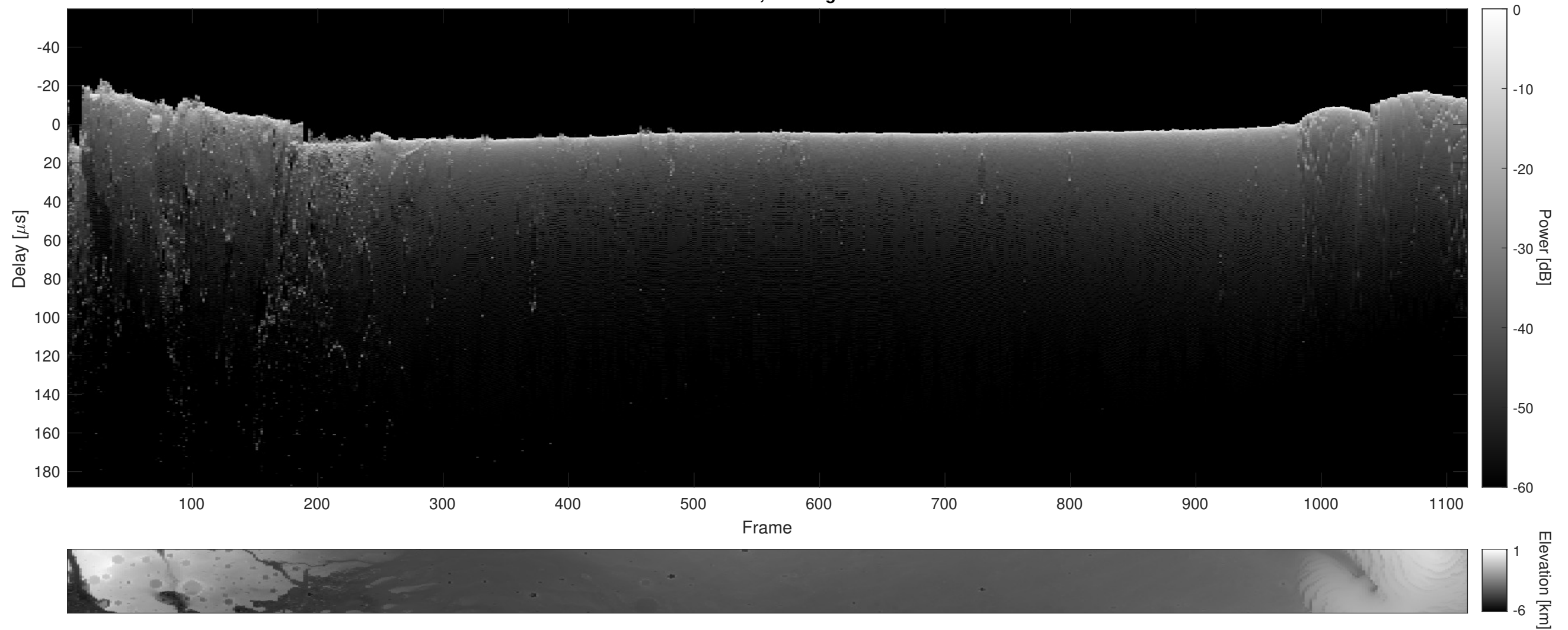
Orbit 12152, Cluttergram
