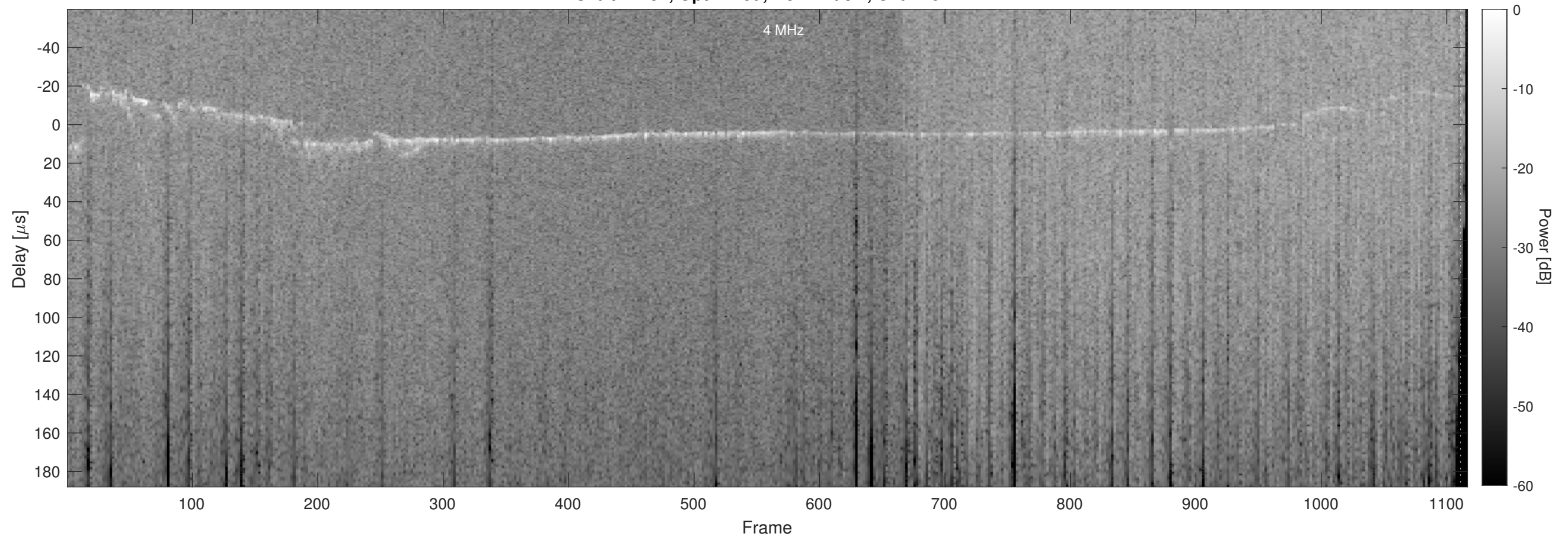
Orbit 12152, Optimized, No Window, Channel 2
