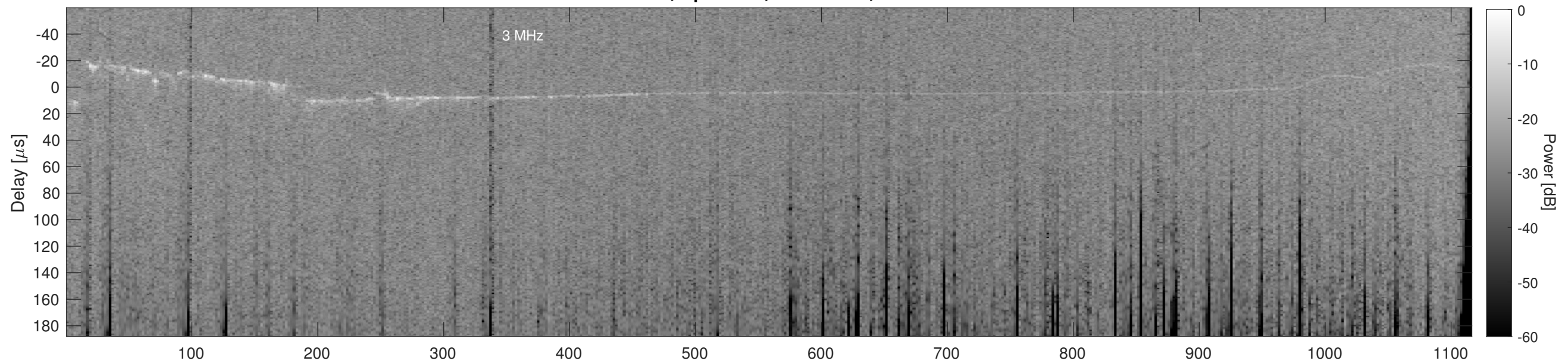
Orbit 12152, Cluttergram
