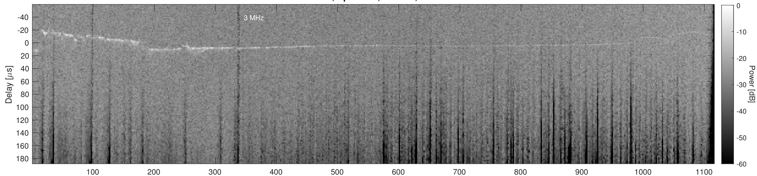
Orbit 12152, Cluttergram
