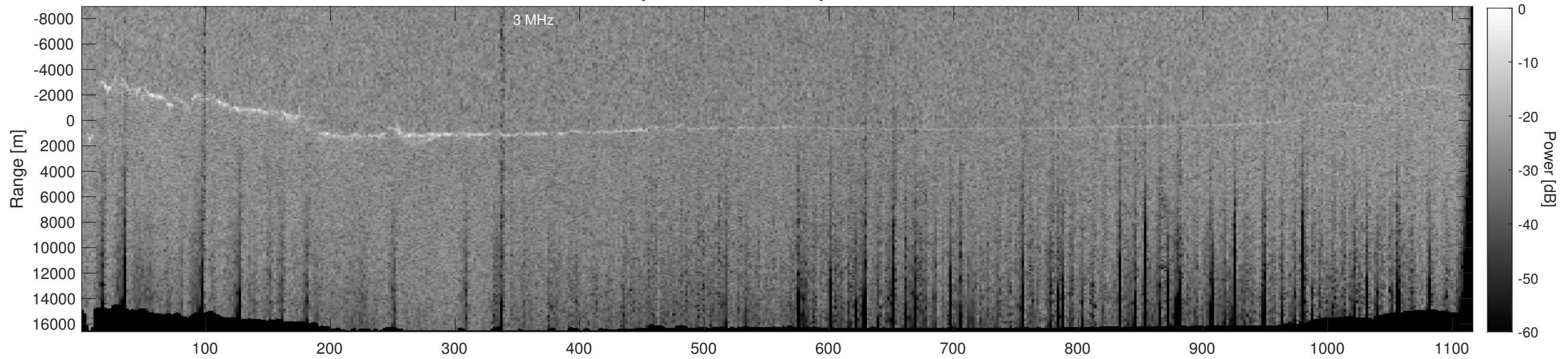
Orbit 12152, Depth-Corrected Cluttergram
