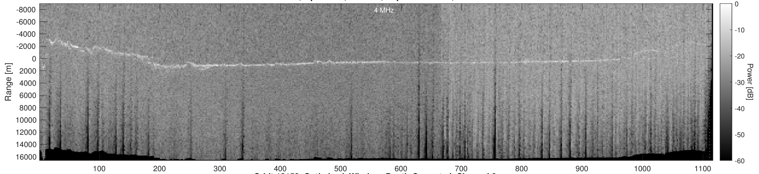
Orbit 12152, Optimized, Window, Depth-Corrected, Channel 2
