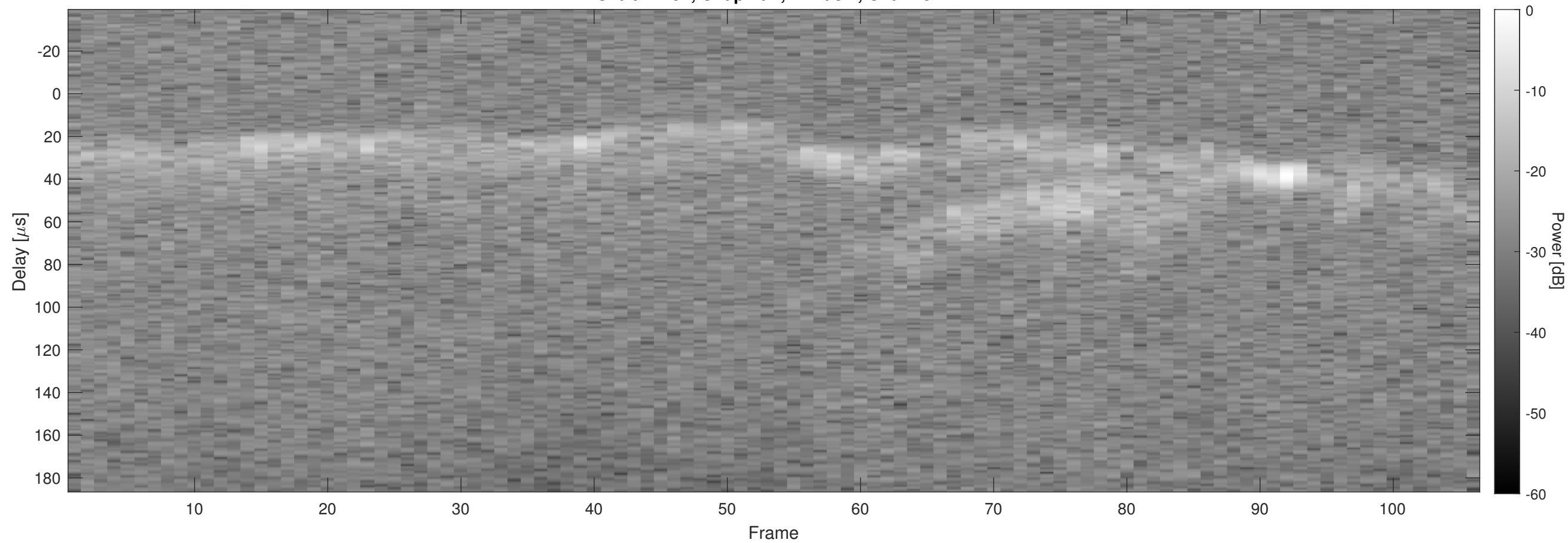
Orbit 12154, Chapman, Window, Channel 2
