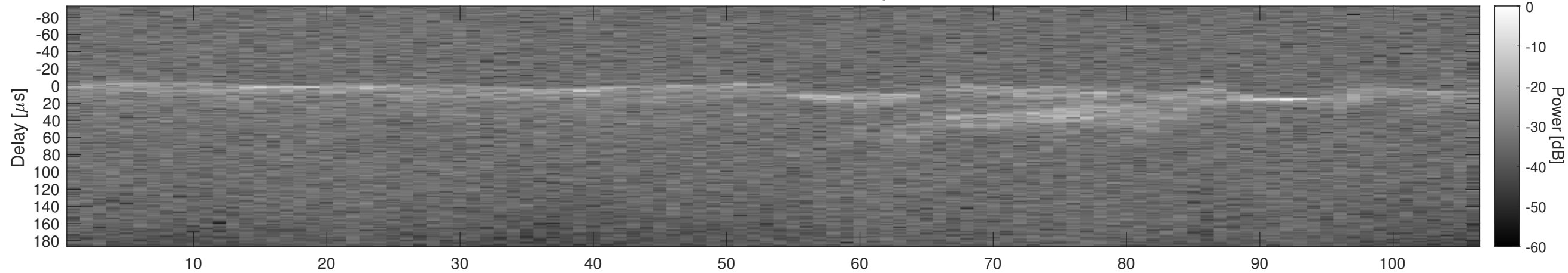
Orbit 12154, Cluttergram
