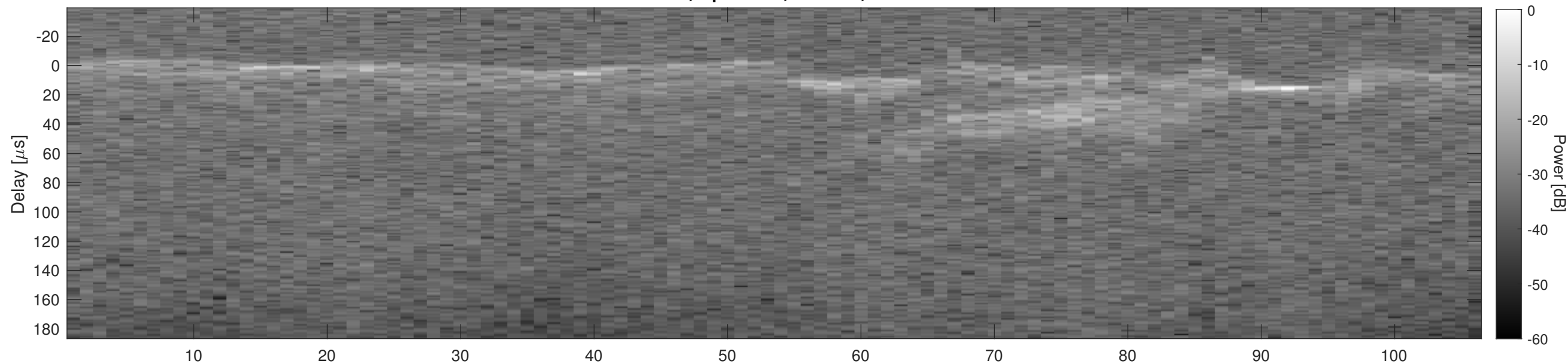
Orbit 12154, Cluttergram
