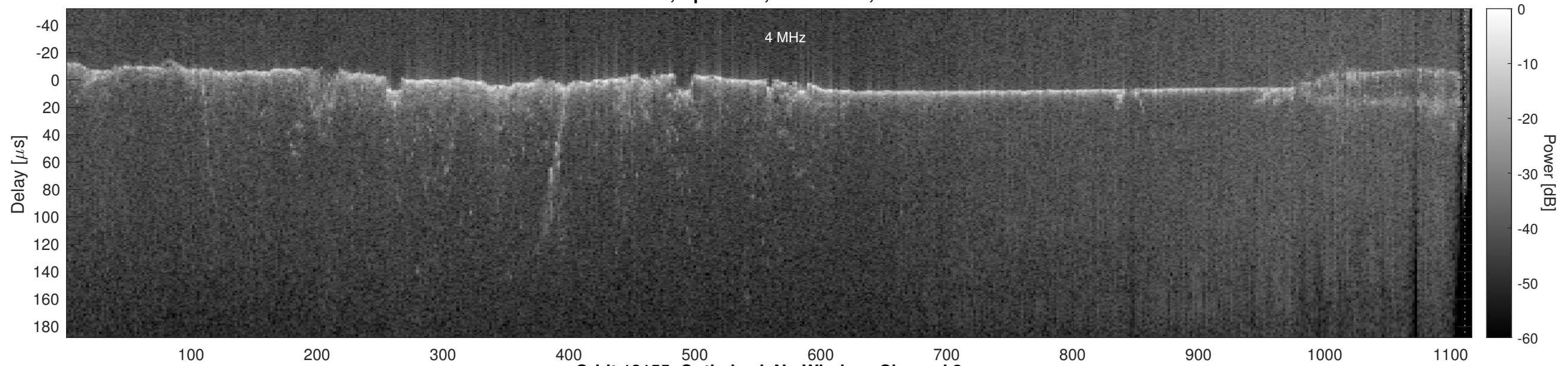
Orbit 12155, Optimized, No Window, Channel 2
