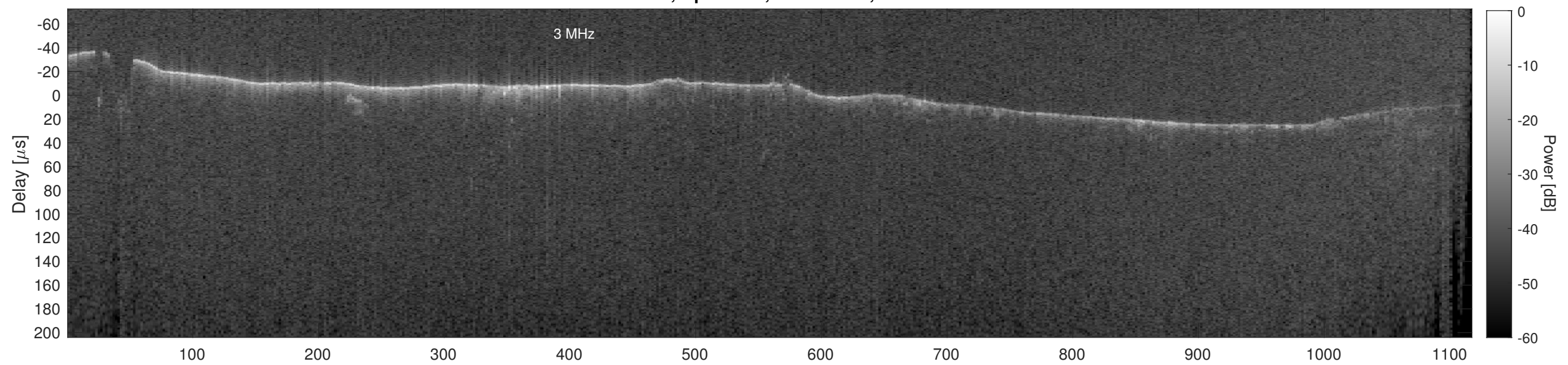
Orbit 12156, Cluttergram
