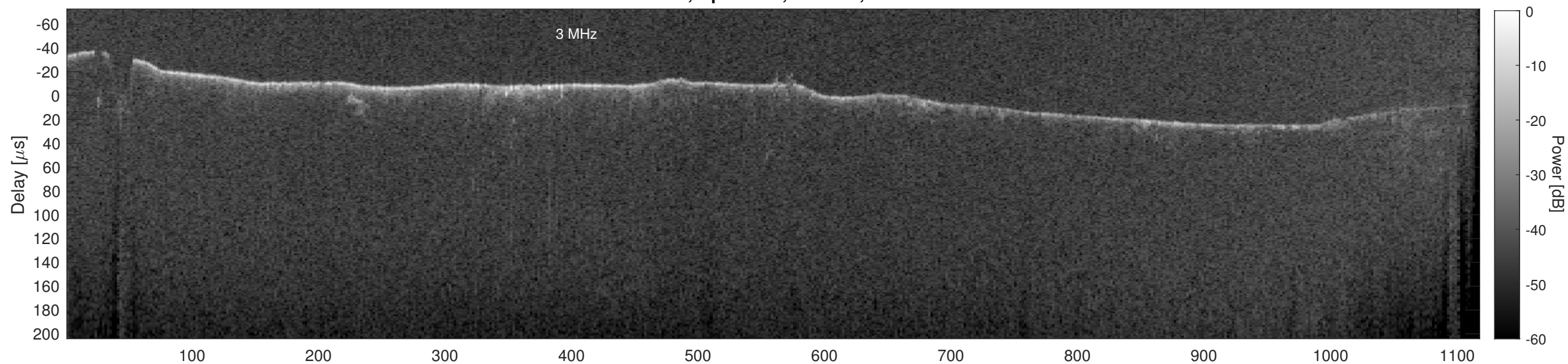
Orbit 12156, Cluttergram
