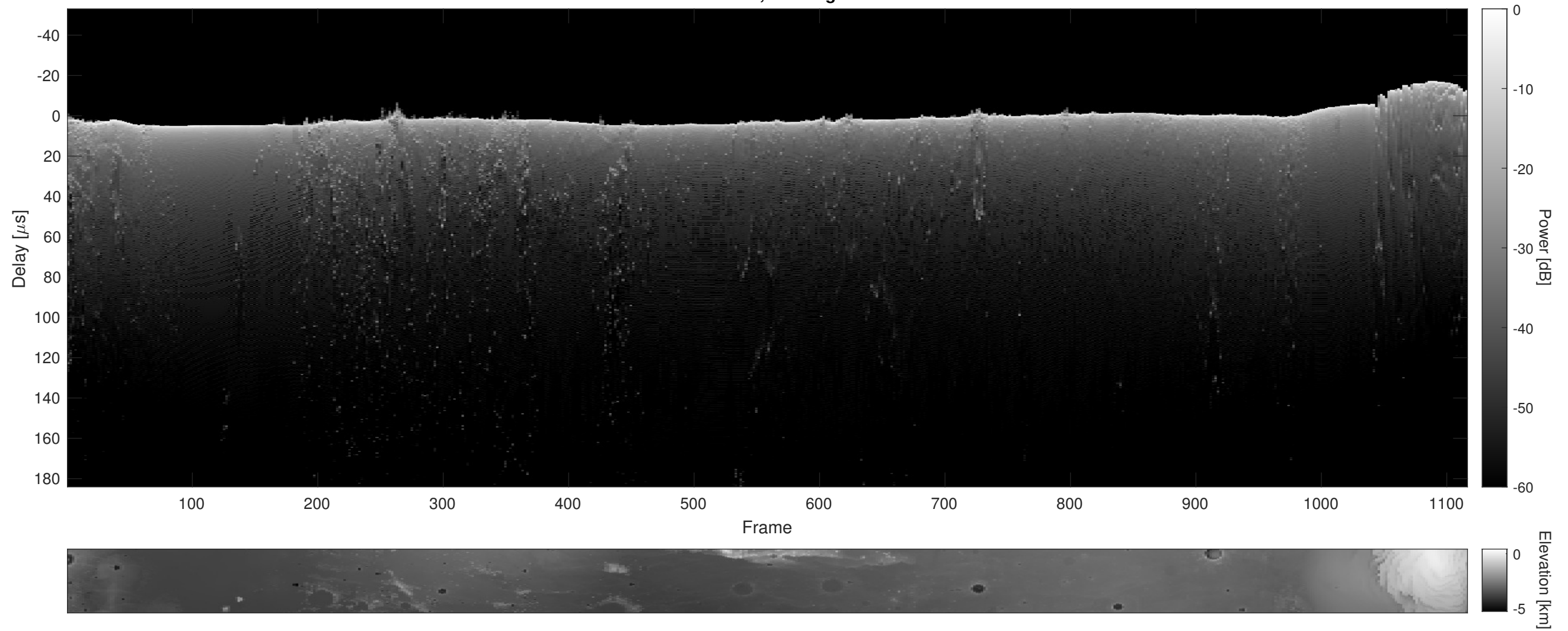
Orbit 12157, Cluttergram
