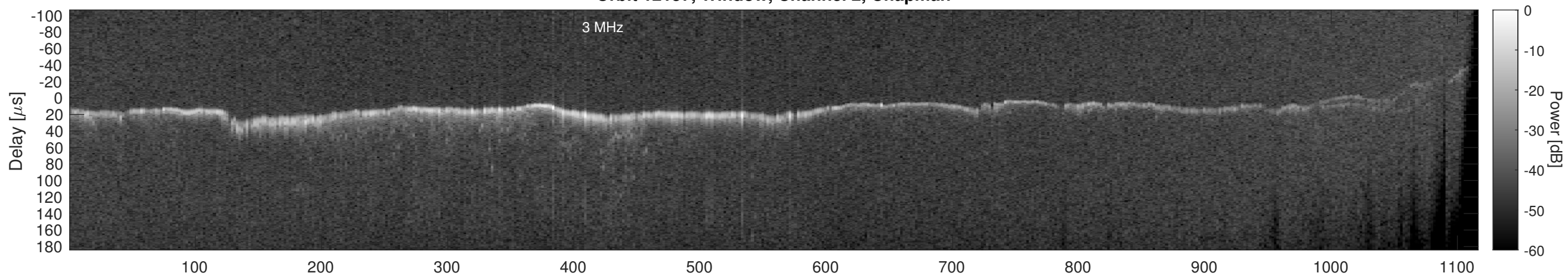
Orbit 12157, Window, Channel 2, Optimized
