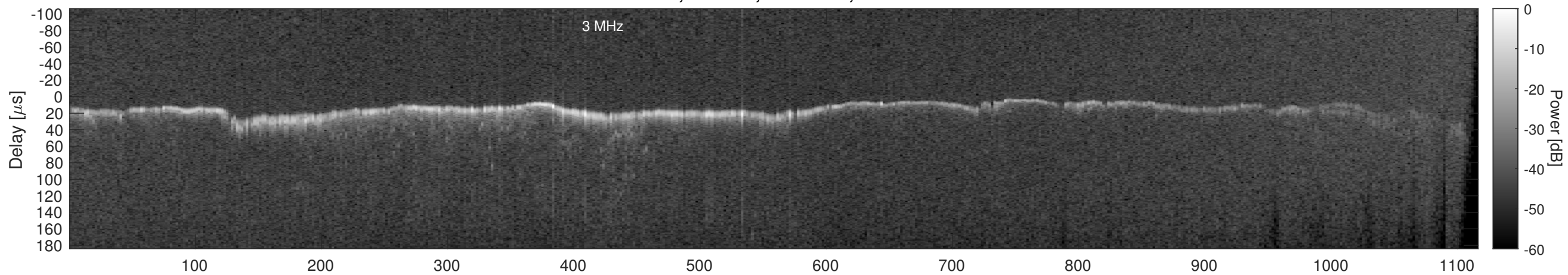
Orbit 12157, Window, Channel 2, Chapman
