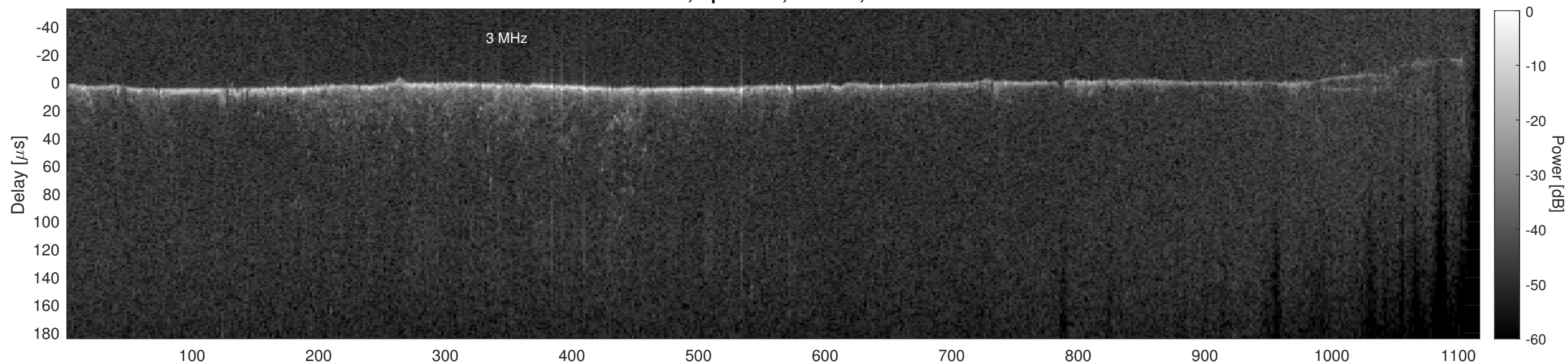
Orbit 12157, Cluttergram
