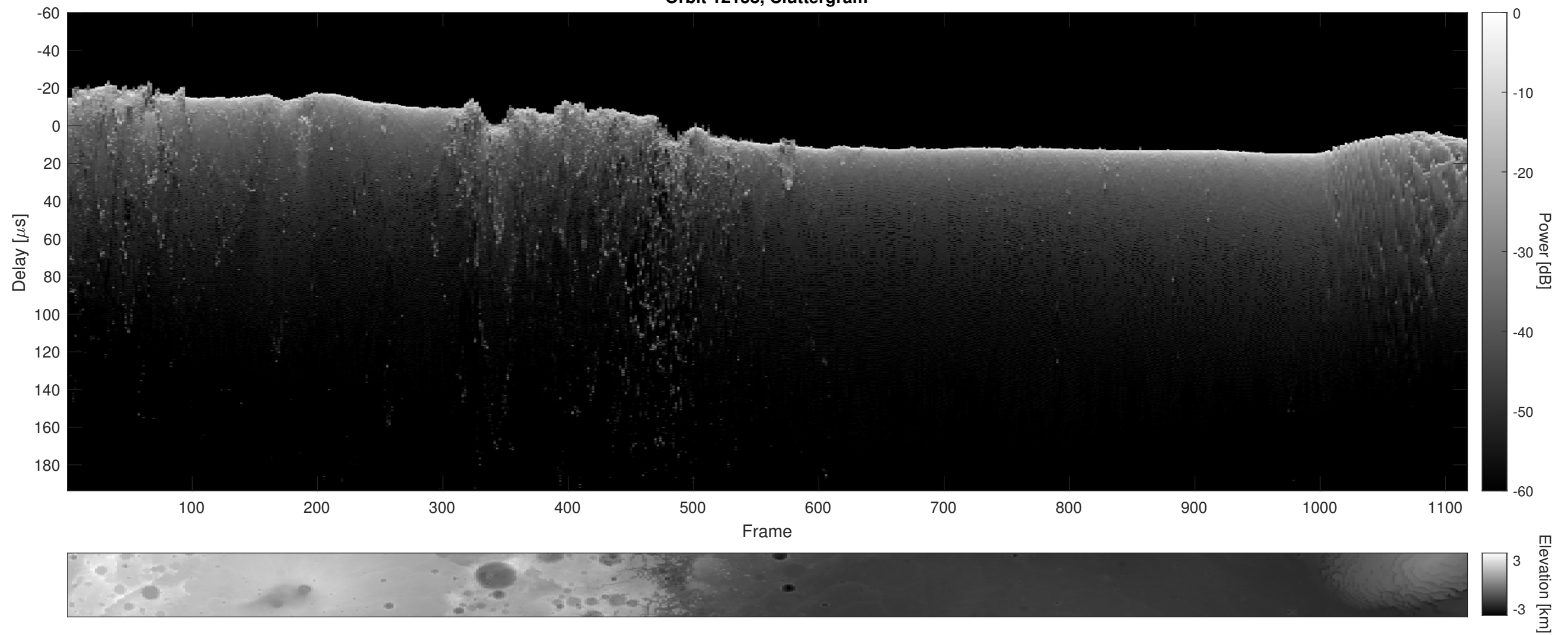
Orbit 12158, Cluttergram
