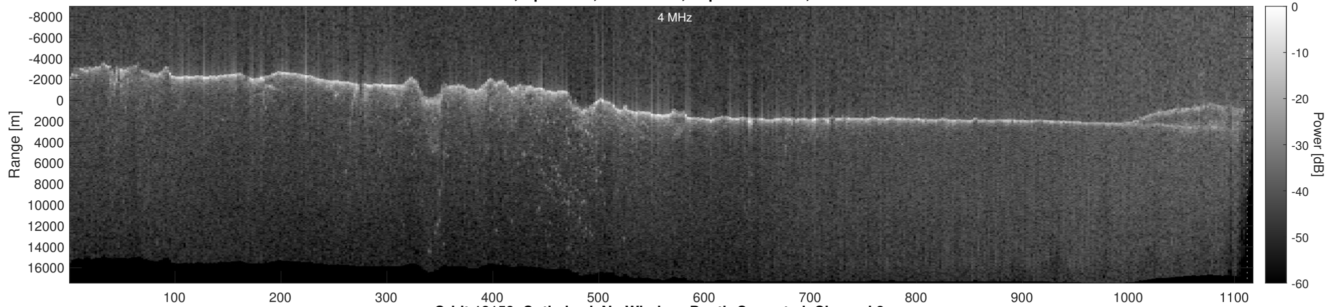
Orbit 12158, Optimized, No Window, Depth-Corrected, Channel 2
