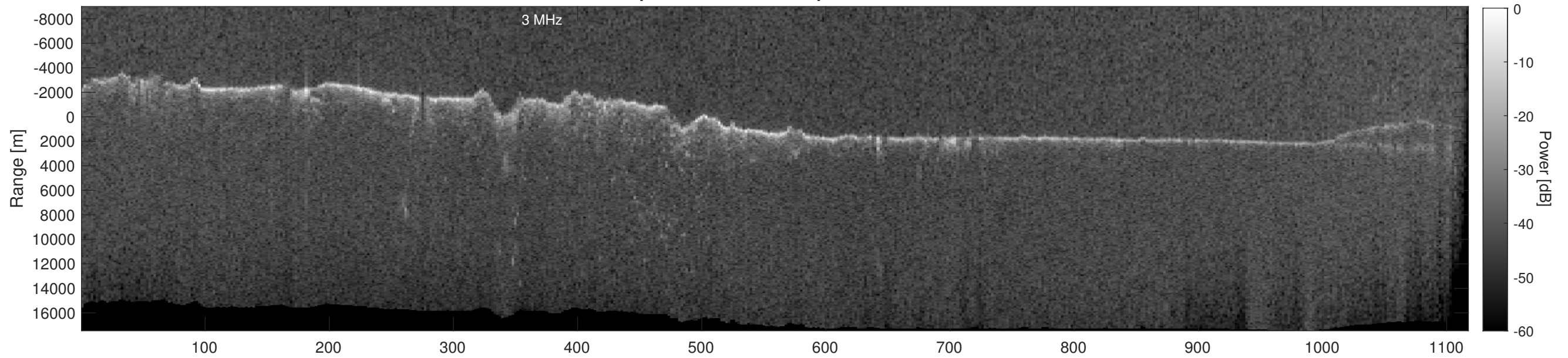
Orbit 12158, Depth-Corrected Cluttergram
