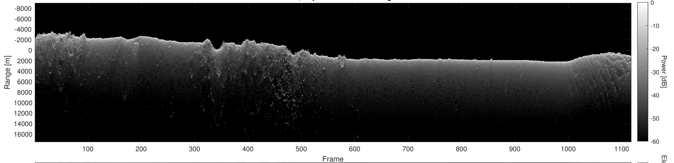
Orbit 12158, Depth-Corrected Cluttergram
