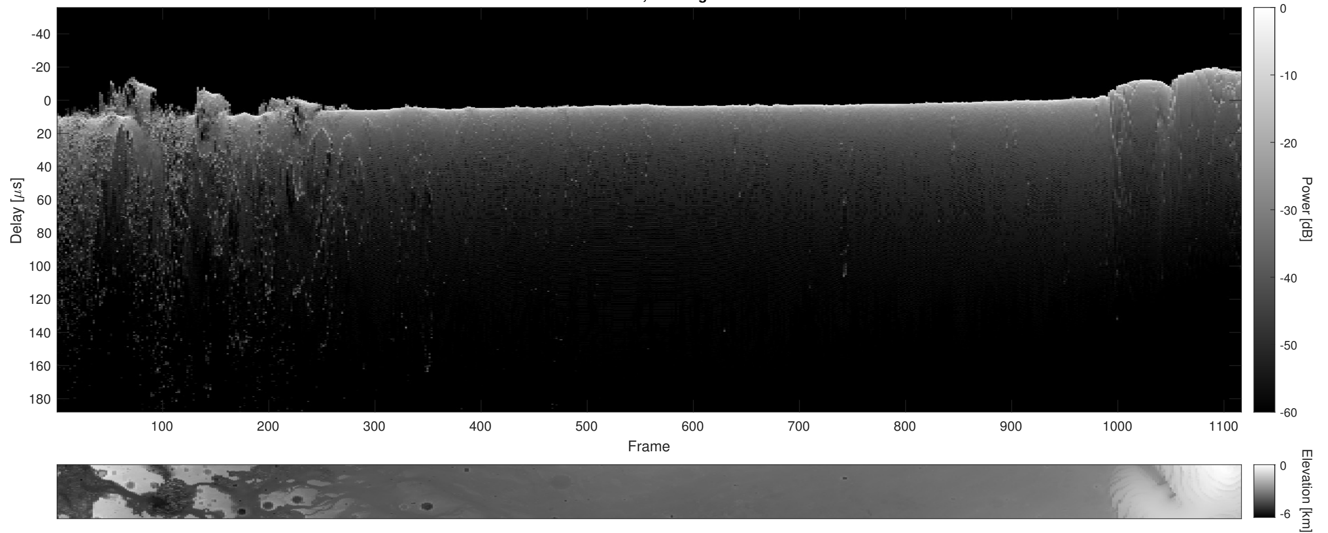
Orbit 12159, Cluttergram
