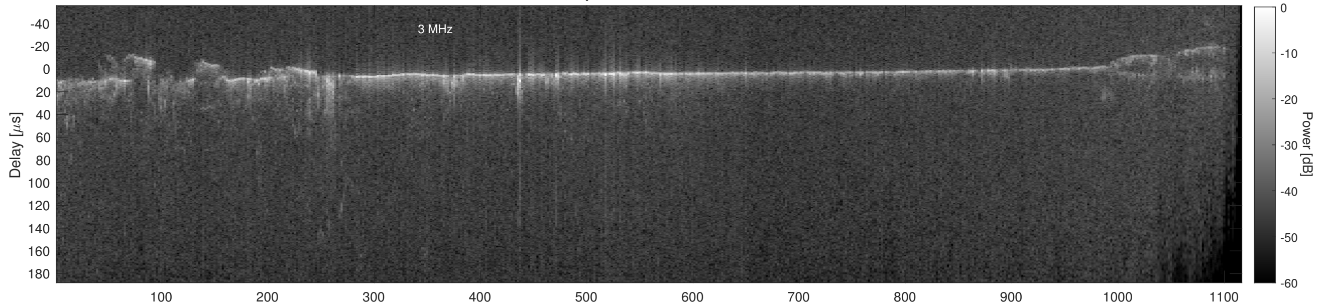
Orbit 12159, Cluttergram
