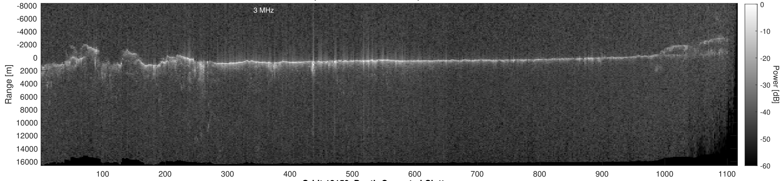
Orbit 12159, Depth-Corrected Cluttergram
