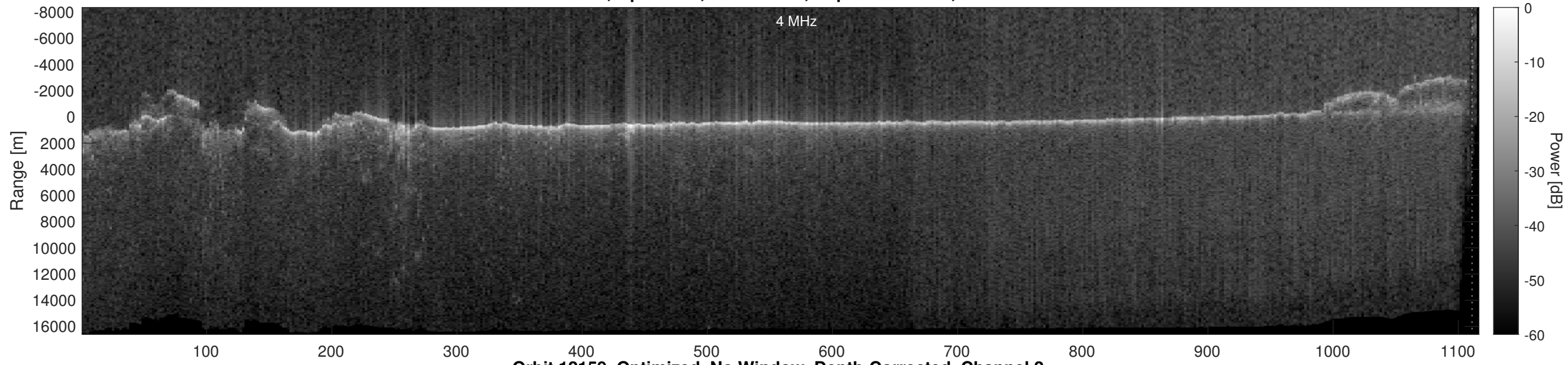
Orbit 12159, Optimized, No Window, Depth-Corrected, Channel 2
