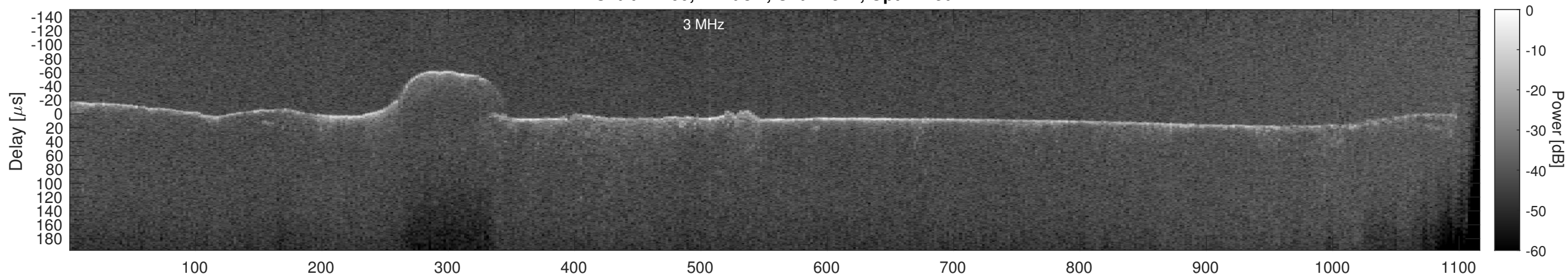
Orbit 12160, Cluttergram
