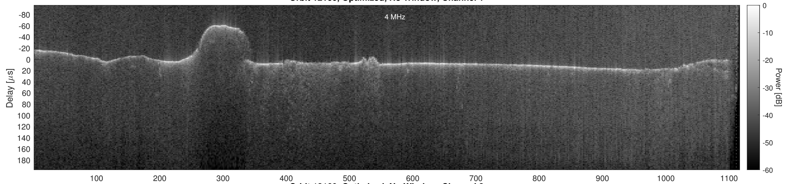
Orbit 12160, Optimized, No Window, Channel 2
