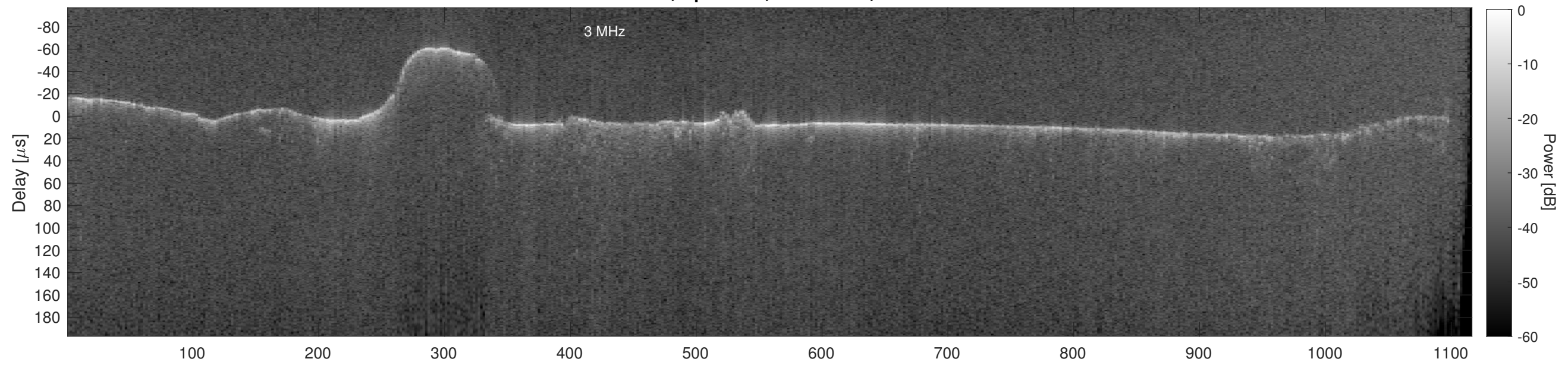
Orbit 12160, Cluttergram
